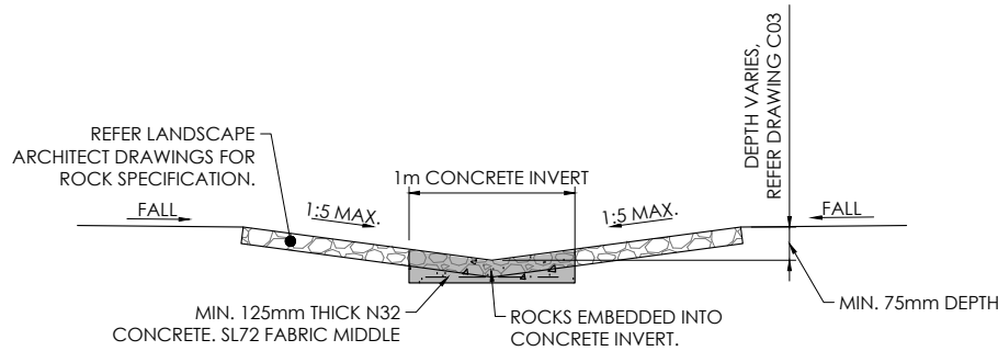
CHANNEL A - TYPICAL DETAIL SCALE 1:50
