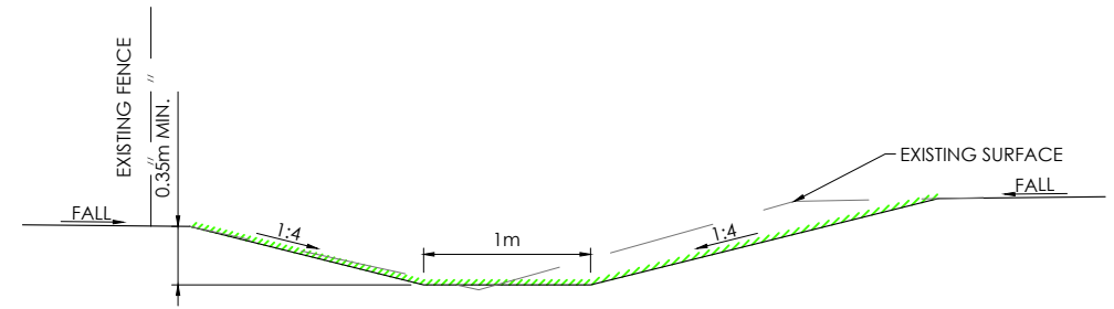
EXISTING RE-PROFILED CHANNEL TYPICAL DETAIL SCALE 1:50
