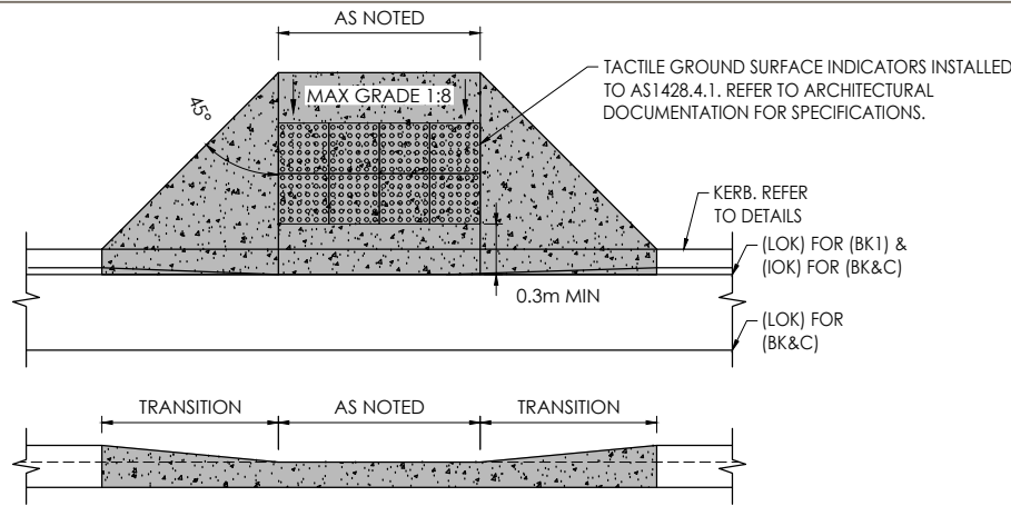
KERB RAMP DETAIL KERB RAMP TO COMPLY WITH AS1428.1 SCALE 1:50
