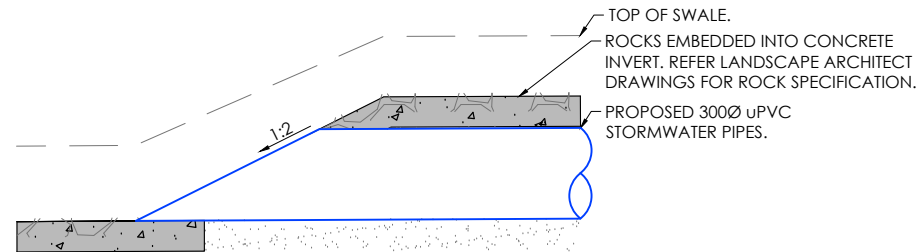
STORMWATER PIPE OUTLET SECTION SCALE 1:25
