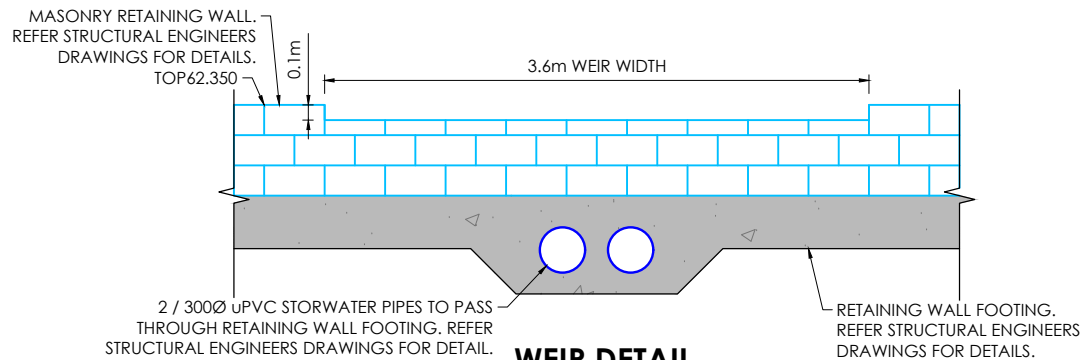
WEIR DETAIL SCALE 1:50
